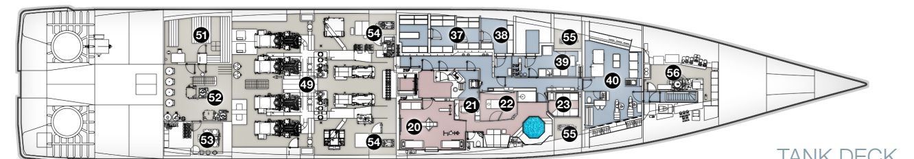
TANK DECK
